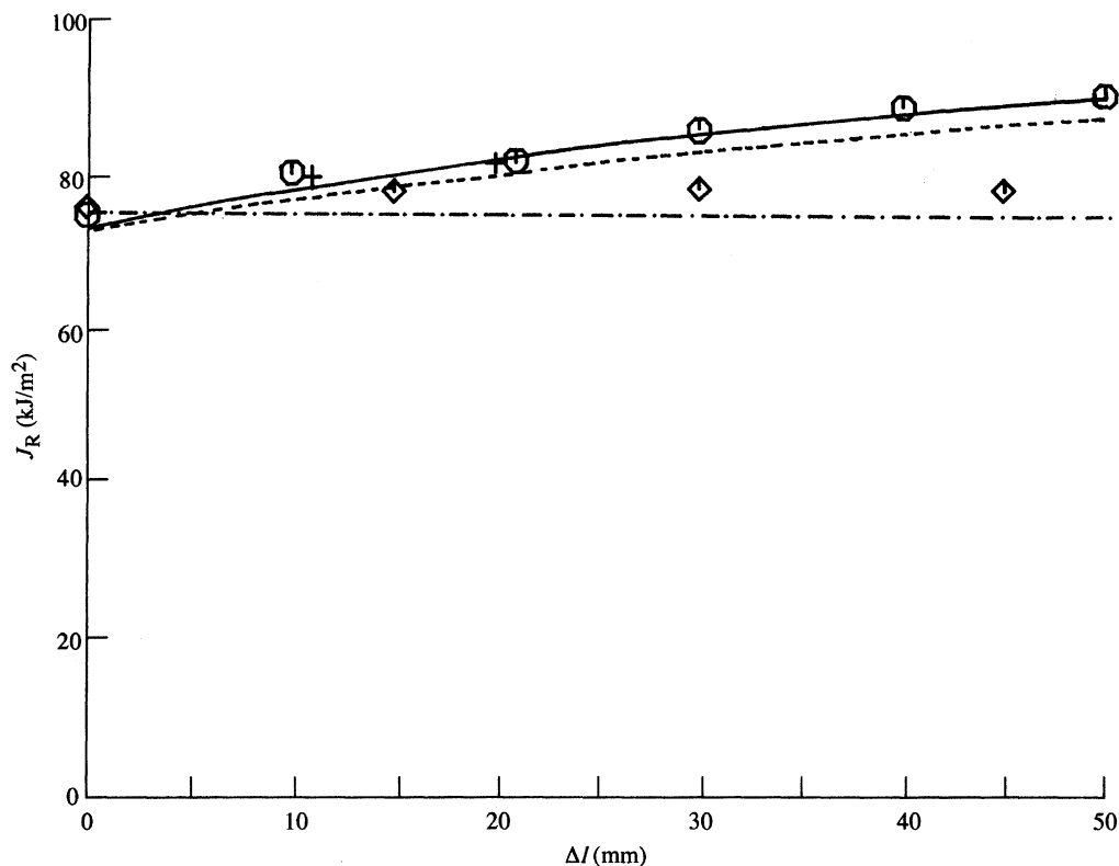
Figure 9. J_R curves for the brass DCB specimens.
