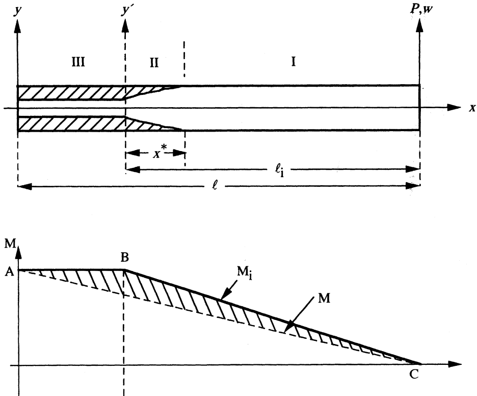
Figure 3. Unloading of an arm of a DCB specimen during equilibrium crack propagation and the three regions of deformation. During crack propagation from \ell_i to \ell the load decreases from P_i to P giving partial unloading of the cantilever arms. The height of the shaded are ABC represents the history of elastic unloading moments behind the crack tip.
