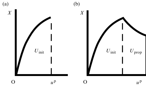
Fig. 1 (a) Irrecoverable work U_{init} up to crack initiation in rigid plastic fracture. (b) Irrecoverable work accumulated during crack propagation in rigid plastic fracture. U_{acc} = U_{init} + U_{prop} .
