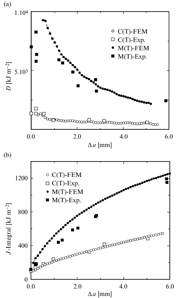
Fig. 2 Typical shapes of (a) energy dissipation rate D curves, (b) J_R curves for StE460 ferritic steel [after (3)].
