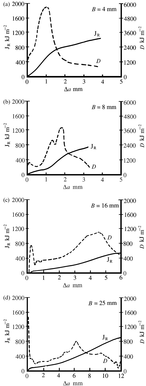
Fig. 8 J_R and D curves derived from the same data by Stampfl and Kolednik 21 in different thickness plates of V720 steel.
