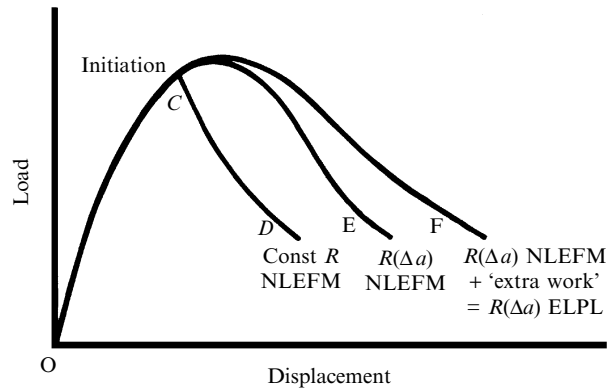
Fig. 6 Schematic relation between the NLEFM initiation solution and subsequent possible propagation paths. Initiation at point C; propagation according to NLEFM at constant toughness R=J_c along CD; propagation according to NLEFM with R(\Delta a) given by Eq. (31) along CE; and ELPL propagation along CF. The additional displacements along CF, in comparison with those along CE at the same load, indicate the ‘extra work’ requirement.
