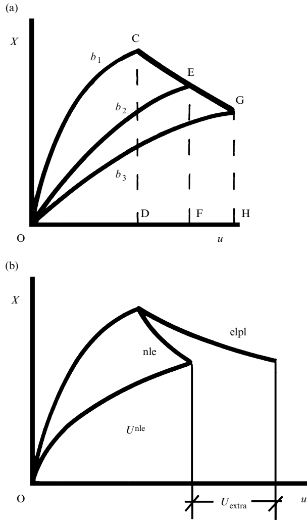
Fig. 3 (a) Load-displacement-ligament-crack length plots for path-independent displacement-reversible NLEFM. (b) For path-dependent, displacement-irreversible ELPL cracking, showing the extra displacement and extra work required to ‘convert’ the NLEFM solution to the practical ELPL problem.
