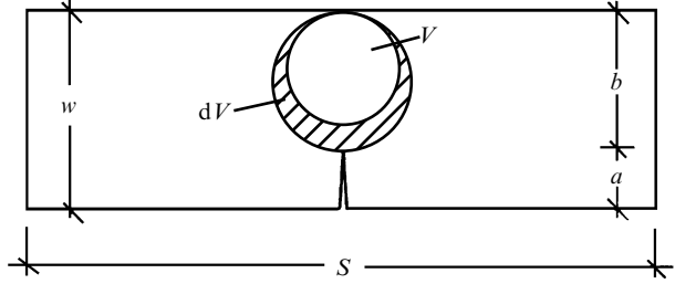
Fig. 4 The incremental volume dV from which energy is fully recovered in nle fracture, but not in ELPL propagation.
