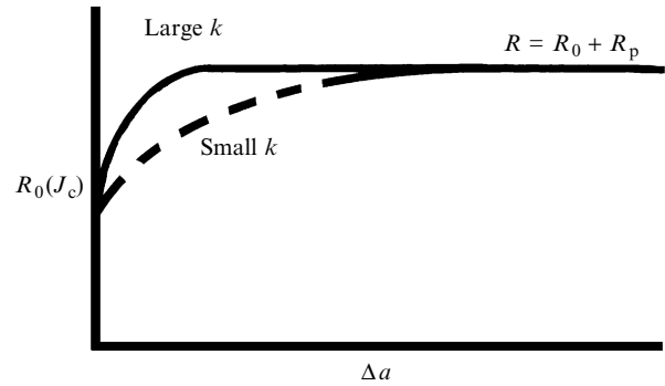
Fig. 5 The change of crack-tip resistance to cracking described by R(\Delta a) = R_0 + R_p [1 - \exp(-k\Delta a)] . Saturation occurs when (if) steady-state is achieved, when shear lip formation, etc. is fully developed.
