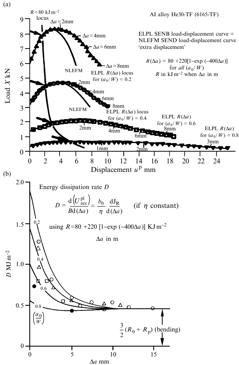
Fig. 7 (a) X-u-a results for side grooved three-point bend testpieces of HE30TF (6165) aluminium alloy with W = 50 mm, B = 12.5 mm, B_n = 6.3 mm, S = 200 mm having (a_0/W) = 0.2, 0.4, 0.6 and 0.8 . Curves are theoretical predictions for X-u-a employing R = 80 + 220 [1 - \exp(-400 \Delta a)] \text{ kJ m}^{-2} ( \Delta a in m). All initiation points (indicated by arrows) lie on the constant R = 80 \text{ kJ m}^{-2} NLEFM locus. (b) D curves for the same (a_0/W) . Note the slight dip in the D curve for (a_0/W) = 0.8 where a minimum is displayed, lower than the final levelled-out value for D . Curves are predictions of Eq. (33) when R = 80 + 220 [1 - \exp(-400 \Delta a)] \text{ kJ m}^{-2} ( \Delta a in m).
