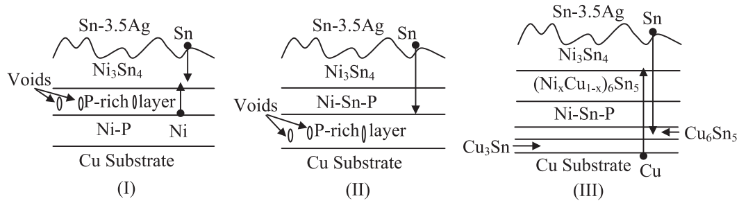
Fig. 5. Schematic illustration for IMC growth in the Sn-3.5Ag/Ni-P/Cu multilayer structure, showing different stages of growth mechanism: (I) formation of thin P-rich Ni-P layer in between Ni 3 Sn 4 and original Ni-P layer during soldering; (II) conversion of P-rich Ni-P layer into Ni-Sn-P layer due to the reaction between Sn and P-rich Ni-P; (III) formation of Cu-Sn and (Ni x Cu 1-x ) 6 Sn 5 IMC due to the reaction between Cu and Sn and between Cu and Ni 3 Sn 4 , respectively.
