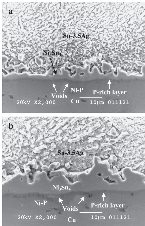
Fig. 3. SEM image of the Sn–3.5Ag/Ni–P/Cu interfaces in the sample annealed at different temperatures for 400 h: (a) 160 and (b) 180 °C.
