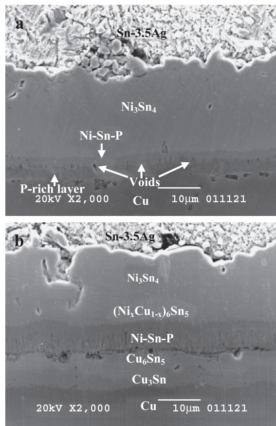
Fig. 4. SEM image of Sn–3.5Ag/Ni–P/Cu interfaces in the sample annealed at 200 °C for (a) 48 and (b) 400 h.
