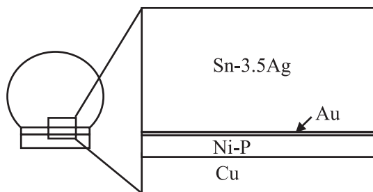
Fig. 1. Schematic diagram of solder joint showing multilayer structure, Sn–3.5Ag/Au/Ni–P/Cu.
