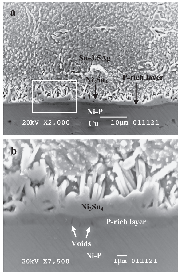
Fig. 2. SEM image of as-prepared sample (a) Sn–3.5Ag/Ni–P/Cu interfaces; (b) magnified view of Sn–3.5Ag/Ni–P interface shown in panel (a) by a rectangle.
