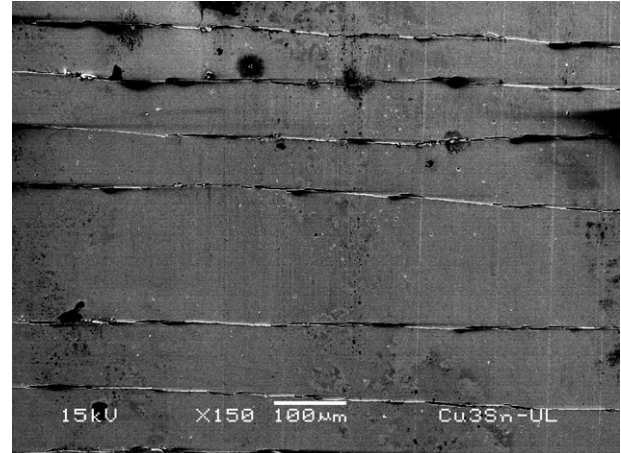
Fig. 5. SEM image of channelling cracks of a Cu–Sn intermetallic thin film.
