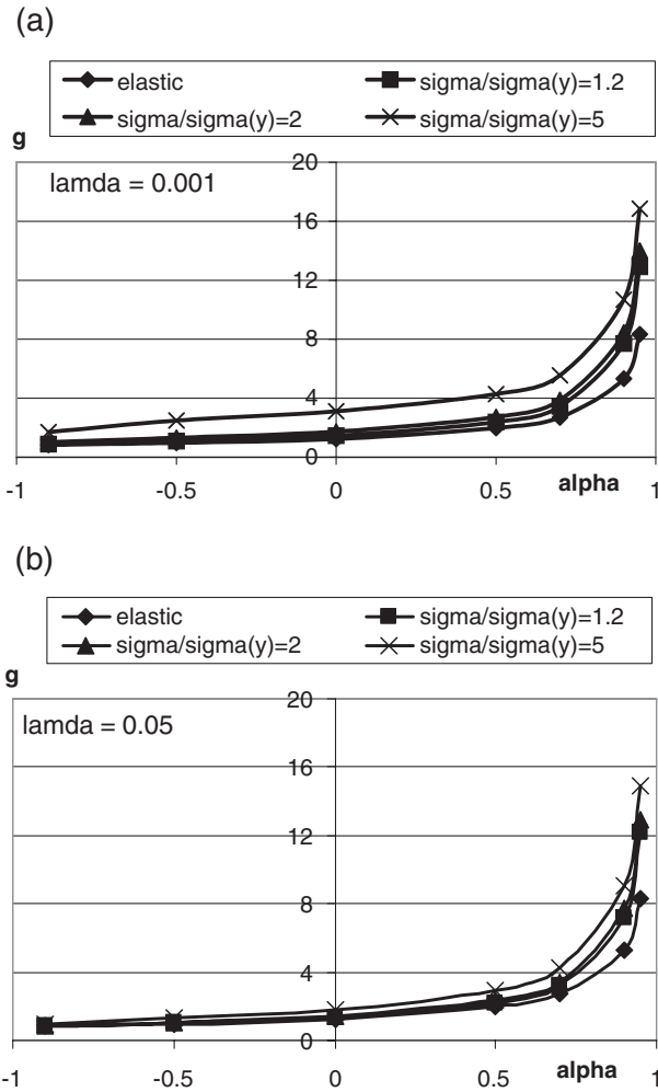
Fig. 3. g(\alpha, \beta, \frac{\sigma}{\sigma_y}, \lambda) versus \alpha for different values of (\sigma/\sigma_y) with \beta=0 . (a) \lambda=0.001 ; (b) \lambda=0.05 .
