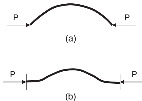
Fig. 1. Schematics of a controlled buckling test. (a) Specimens with simple support (free) ends, (b) specimens with clamped (built-in) ends. The film is always placed on the tension (top) side of the plate.
