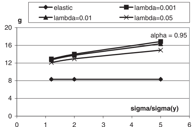
Fig. 4. Effect of (\sigma/\sigma_y) on g(\alpha, \beta, \frac{\sigma}{\sigma_y}, \lambda) at different \lambda 's with fixed \alpha=0.95 .
