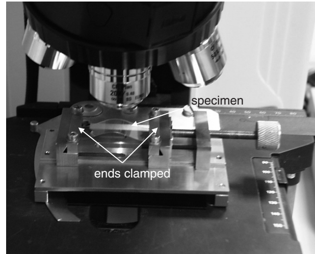
Fig. 2. Controlled buckling test fixture operated manually under an optical microscope. Film cracking can be directly monitored during the experiment.
