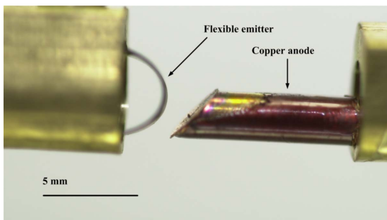
FIG. 2. Field emission measurement of the CNF-based flexible emitter.
