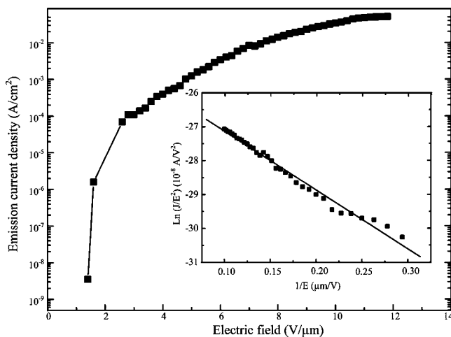
FIG. 2. Field emission measurement of the CNF-based flexible emitter.
