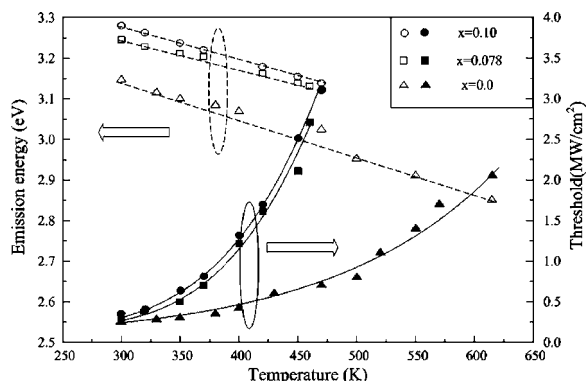
FIG. 4. Temperature dependence of lasing peak emission and lasing threshold of the \text{Zn}_{1-x}\text{Mg}_x\text{O} nanoneedles, for x=0, 0.078 , and 0.1 . The solid line represents the best result of the least-squares fit to the experimental data.
